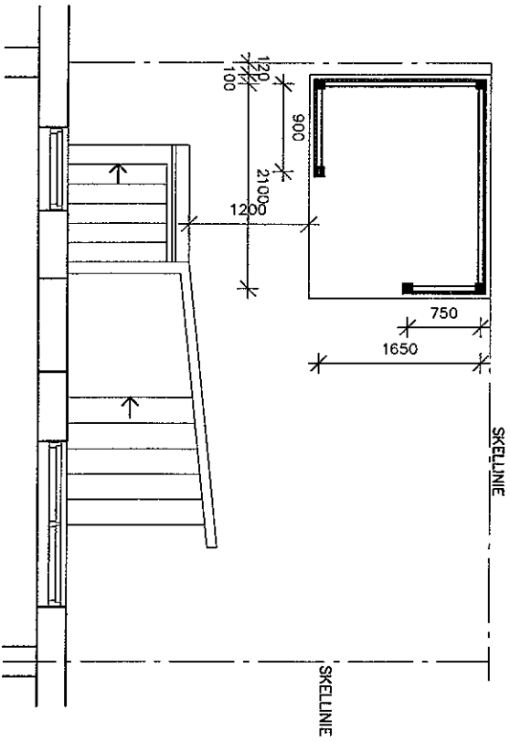
PLAN 1: 1:50
